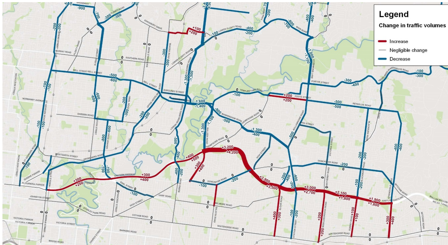
Figure 9-34 Change in average weekday truck volumes (AWDT), 2036 'with project' versus 2036 'no project' – study area south
