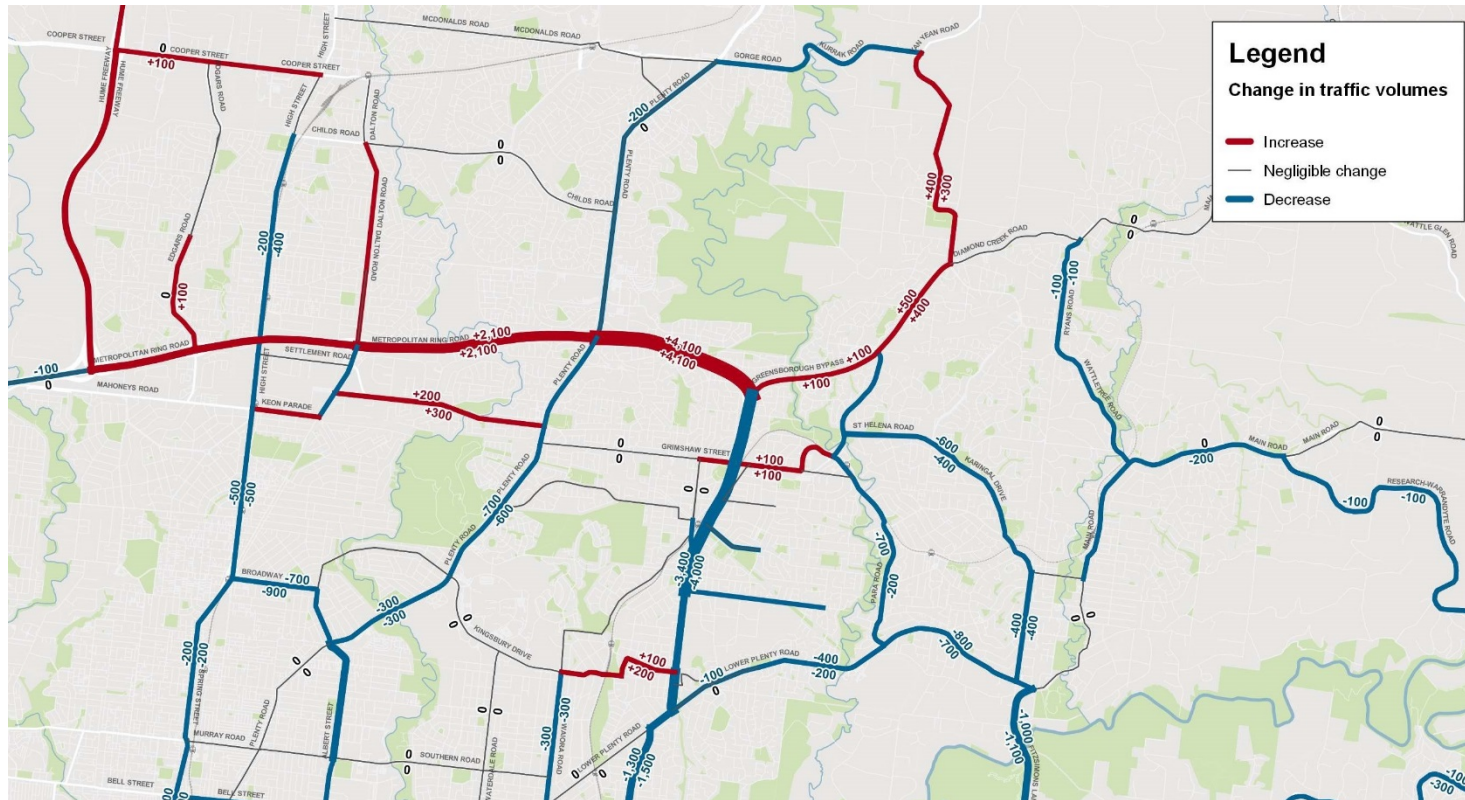
Figure 9-33 Change in average weekday truck volumes (AWDT), 2036 'with project' versus 2036 'no project' – study area north
